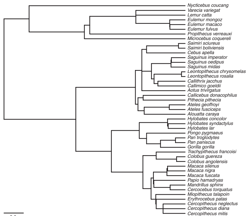
Fig. 1 A phylogenetic tree for the 45 primate species included in this study, derived from Bininda-Emonds et al. (2007, 2008). Branch lengths are scaled to be proportional to time in millions of years.
